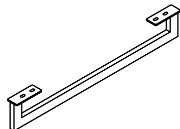
Leg Support 950x50x120MM 2 pcs
